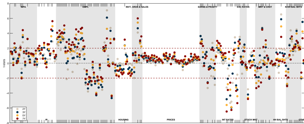
Figure 3.2: Markers indicate t-statistics from logit regressions of the EH state probabilities for maturities n = 2, 3, 5 and 7 on 248 individual macroeconomic variables from the FRED-QD database. Red dashed line indicates \pm 2 for reference. Shading indicates variable groups as defined in the appendix to McCracken and Ng (2016) (See table 3.3).
