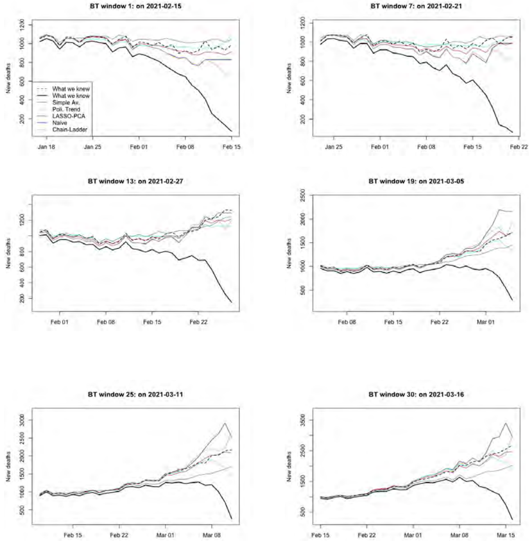
Figure A.4: Six BT windows obtained in the Nowcasting of April 16, 2021. The "Simple Average" model performs exceptionally well and thus receives the highest weight in that actual nowcast window.
