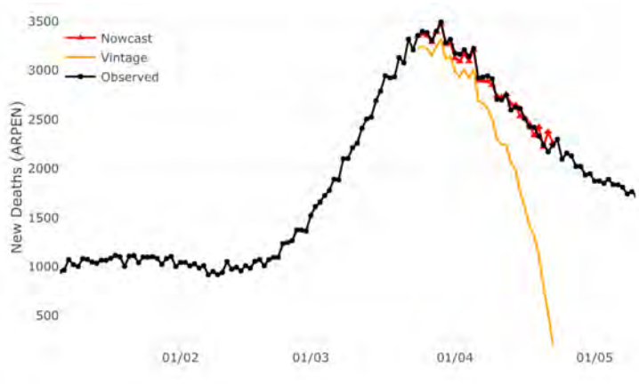
Figure A.7: Nowcast results of its second release on April 23, 2021.
