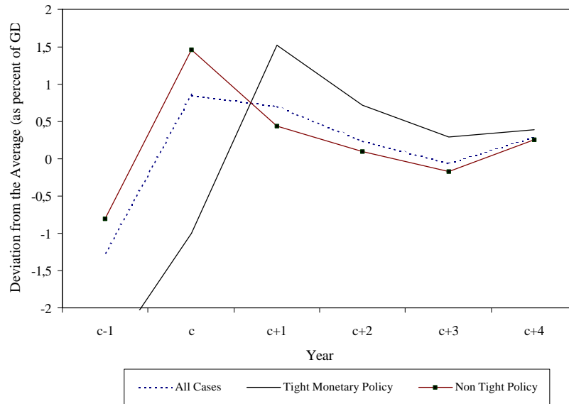
Chart 8: Current Account during and after Undervaluation
