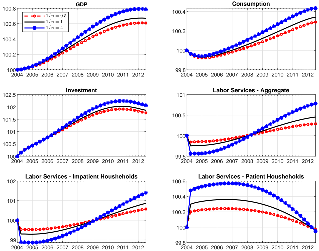
Figure B4: Sensitivity analysis: \varphi .
