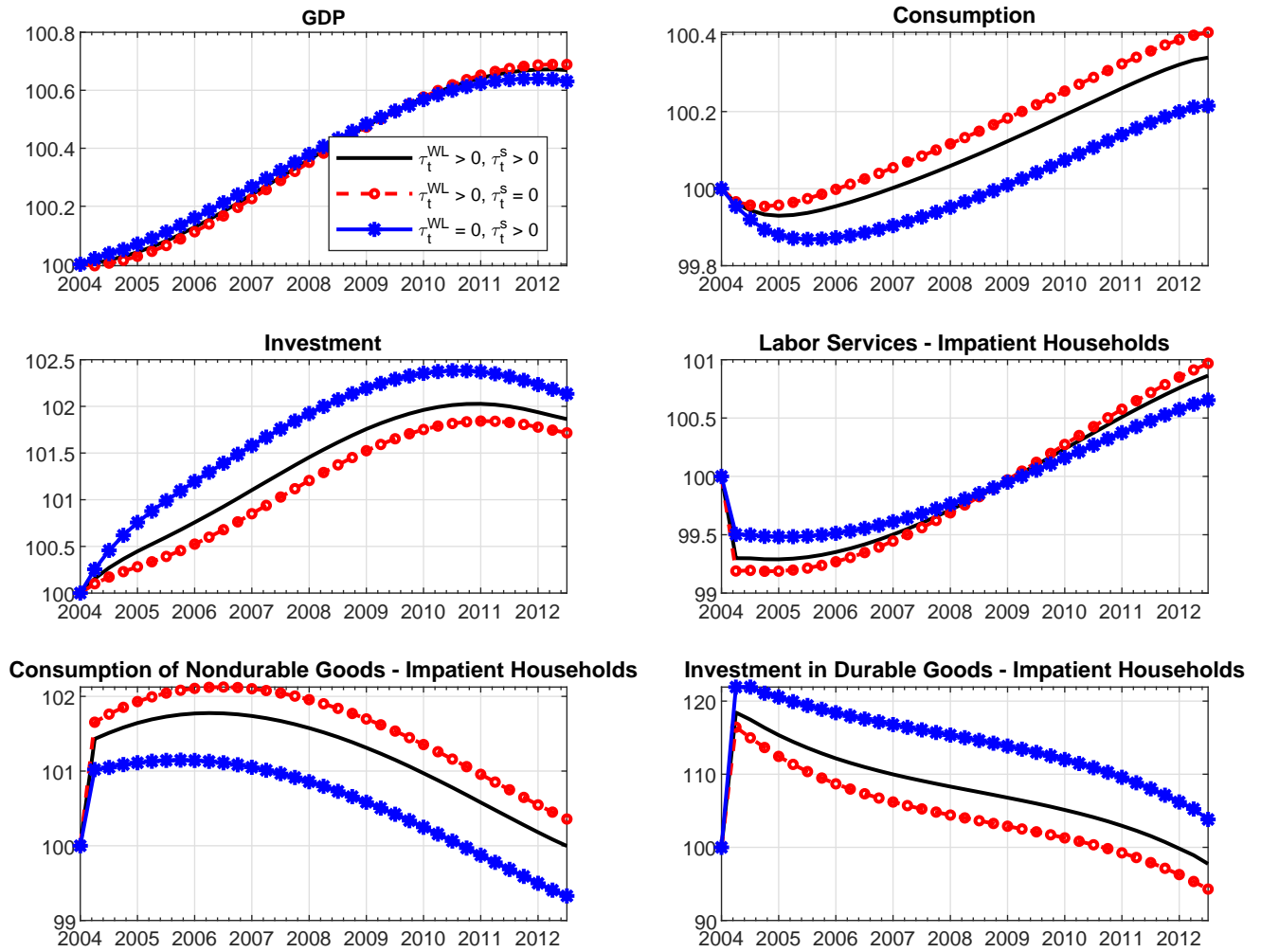
Figure B6: Alternative borrowing constraints: labor income vs. stock of durables.
