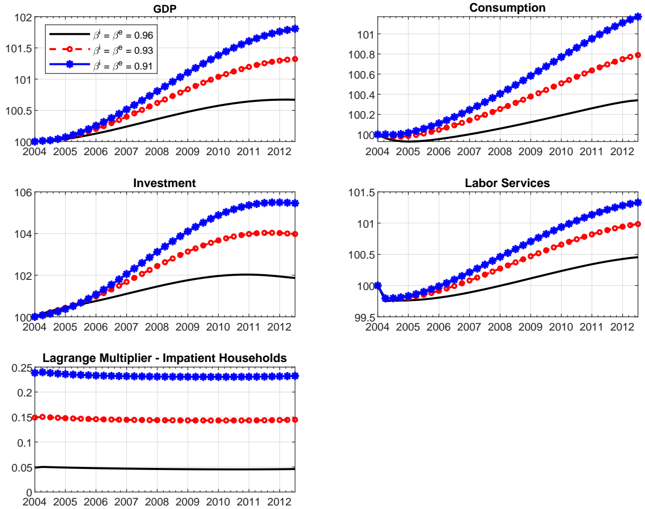
Figure B3: Sensitivity analysis: \beta^e and \beta^i .
